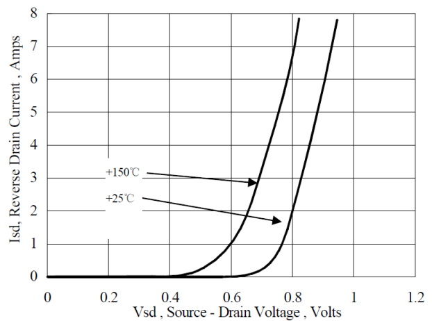
Fig 6 Body-Diode Characteristics
